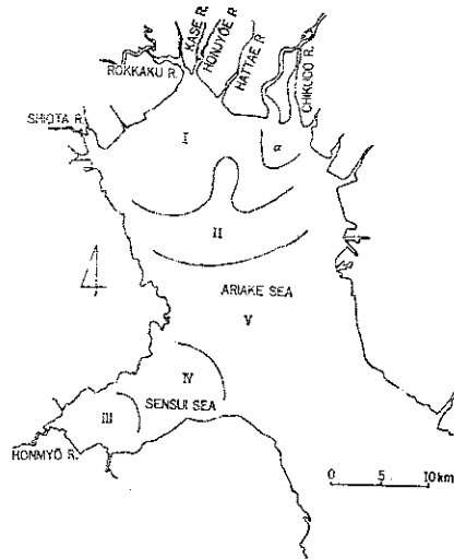
Fig. 6 Distribution of humic acids by using the value P' in the Ariake Sea
