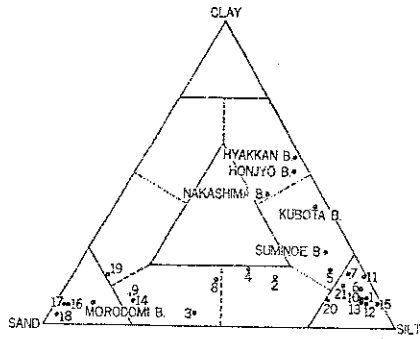
Fig. 4 Classification of sediments based on sand-silt-clay ratio
