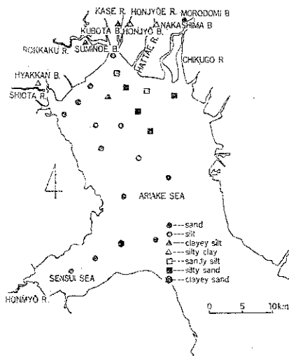
Fig. 5 Classification of sediments based on sand-silt-clay ratio
