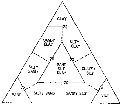
Fig. 3 Nomenclature based on sand-silt-clay percentages (SHEPARD, 1954)
